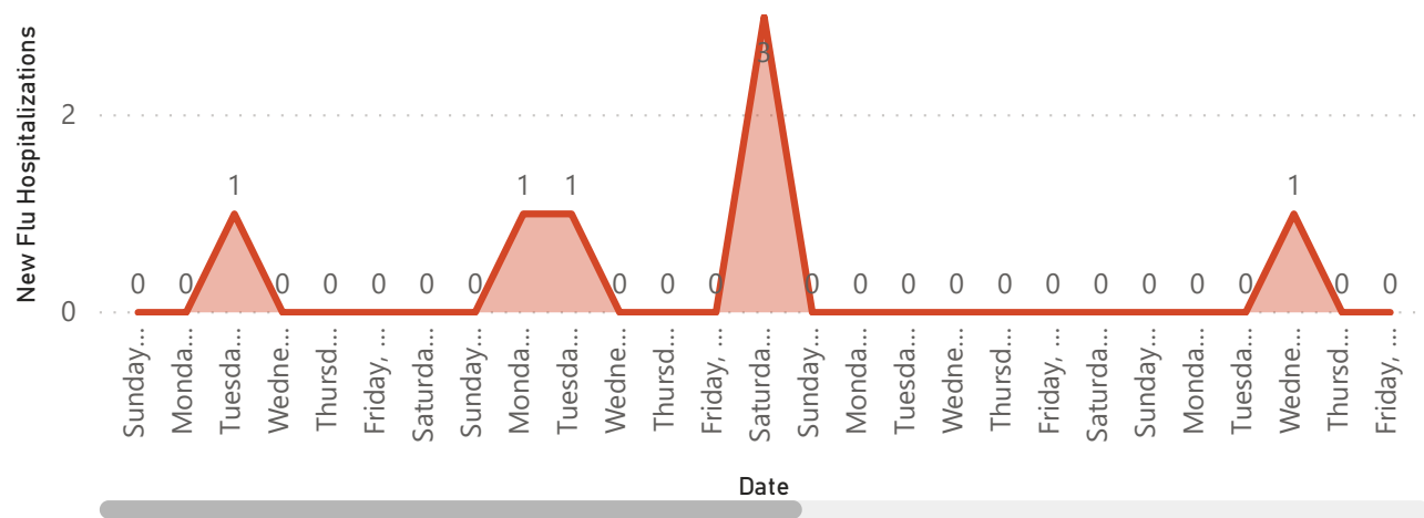
Influenza Hospitalizations, by Date
